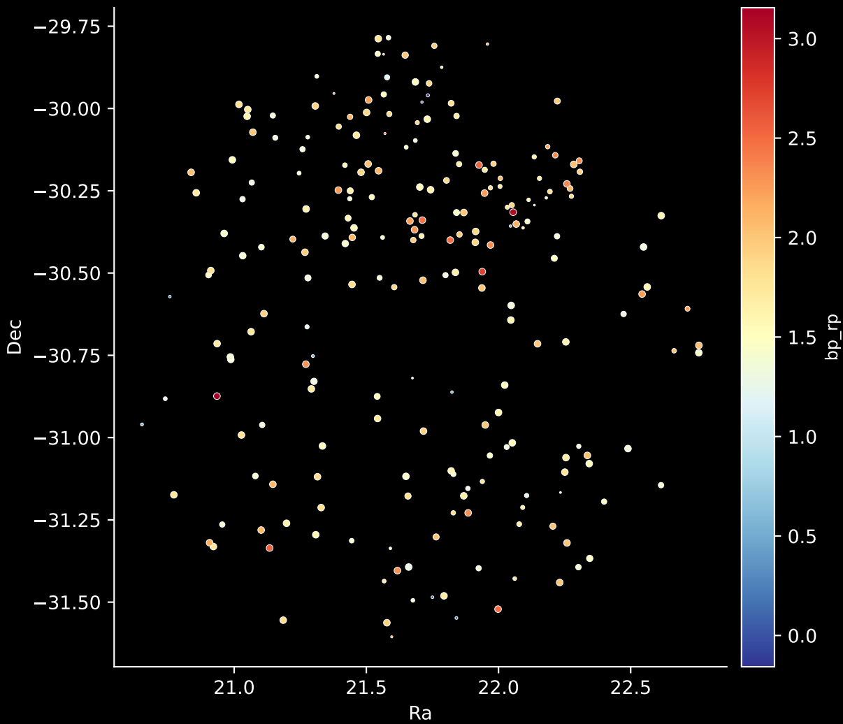
APOGEE DR17 Field: [SGRC-1] Stars: 219
