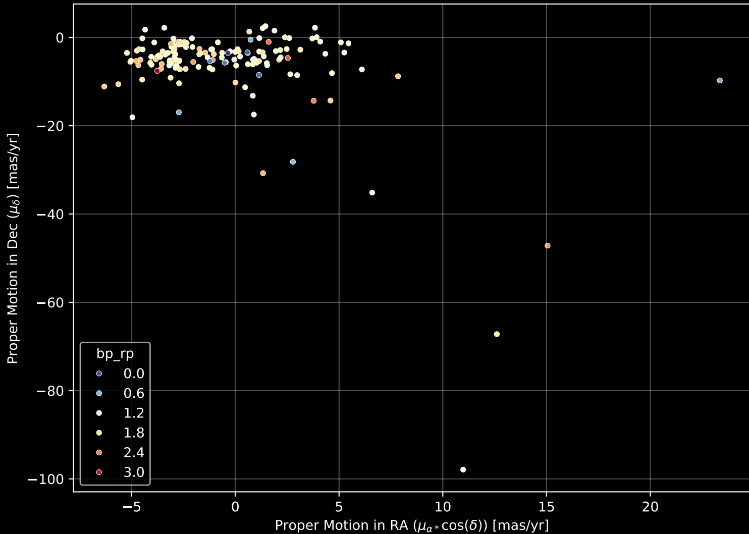
APOGEE DR17 Field: [SGRC-1] Proper Motion Diagram (n= 219)
