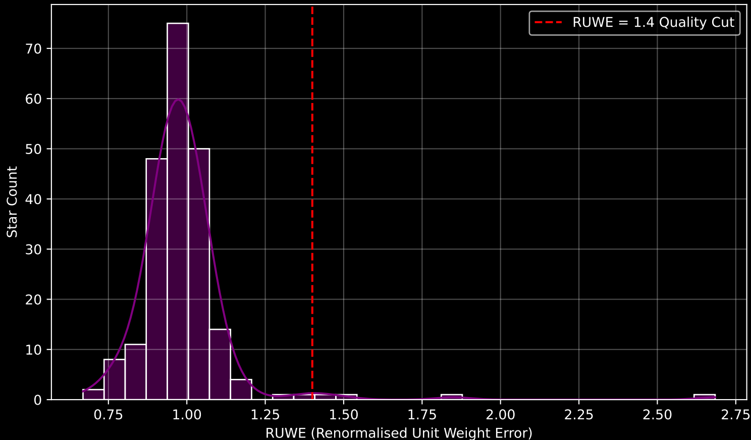
GAPOGEE DR17 Field [SGRC-1] RUWE Distribution (n= 218)
