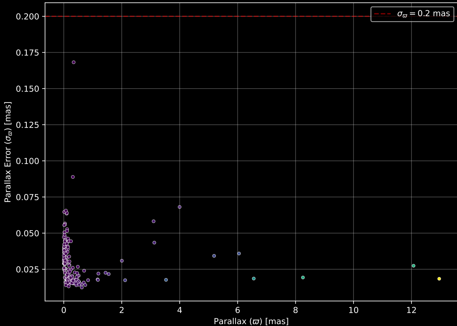
APOGEE DR17 Field: [SGRC-1] Parallax Quality (n= 219)
