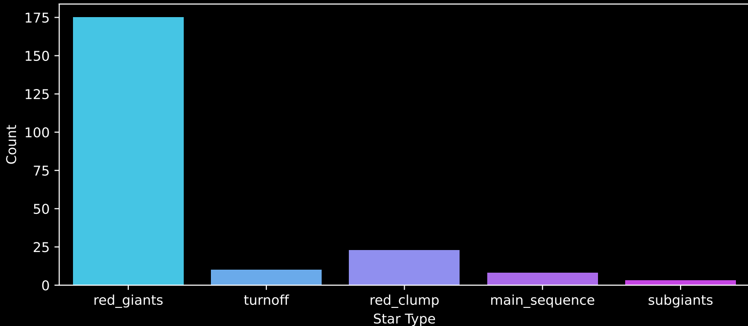
APOGEE DR17 Field: [SGRC-1] Count plot of Star Type
