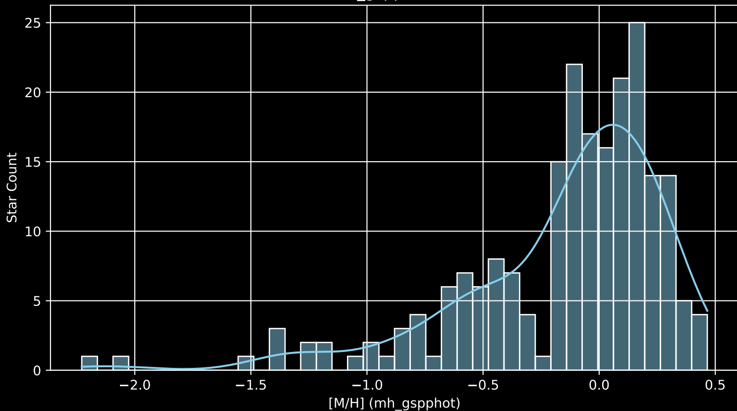
APOGEE DR17 Field: [SGRC-1 [M/H] (mh_gspphot) (n= 214)
