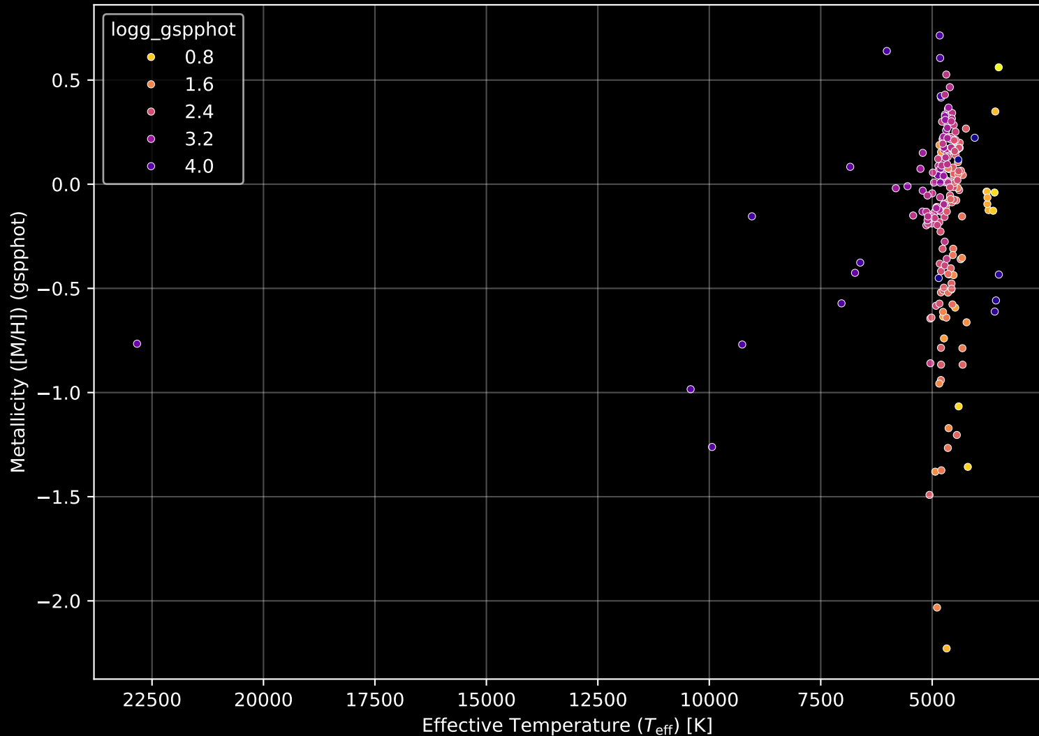
APOGEE DR17 Field: [SGRC-1] Stellar Population Parameters (n= 219)
